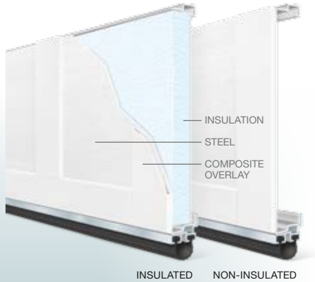
INSULATED NON-INSULATED
